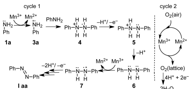
Scheme 2. Proposed mechanism of the reaction.
